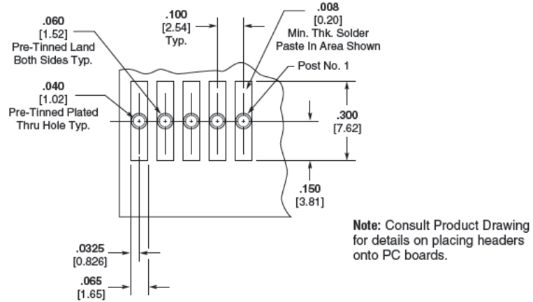
Recommended Mounting Hole Pattern for .062 [1.57] Thick PC Board
